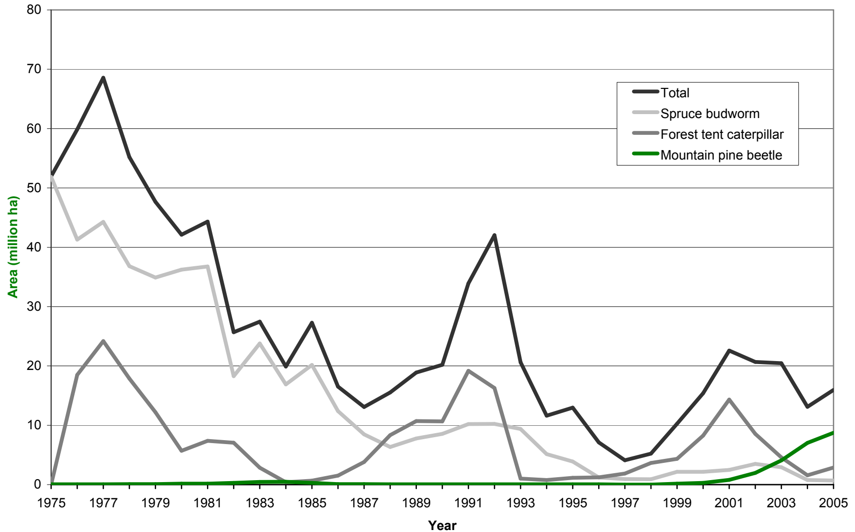
Figure 2.3b Area disturbed by selected insects in Canada (1975–2004) (CCFM, 2007).
